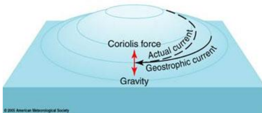
Figure 6: The geostrophic current develops when surface water while flowing downhill balance between the Coriolis force and the force arising from the horizontal water pressure gradient such that surface currents flow parallel to the contours of elevation of sea level ( http://oceanmotion.org/ )
